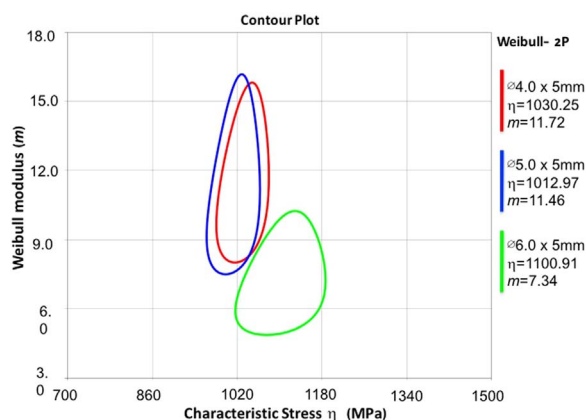
Fig. 1. Contour plot showing “ m ” as an indicator of structural reliability (Weibull modulus) vs. characteristic stress ( \eta ), which indicates the stress in which 63.2% of the specimens of each group may fail. The non-overlap between groups indicates significant difference.
