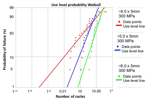
Fig. 2. Use level probability Weibull (90% confidence bound) showing the probability of failure vs. number of cycles for tested groups (set stress 300 MPa).
