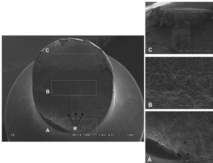
Fig. 3. Shows the fractured abutment. White asterisk represents the origin of the fracture at the surface undergone to tensile stress (A); black arrows indicate the crack propagation direction. When stress suppress the titanium strength, a plastic zone is created and the deformation process takes place (B). At the opposite surface, a rupture zone can be observed at the area subjected to compression stress (C).
