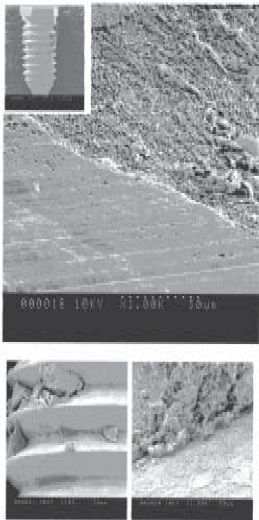
Figure 7A. Scanning electron micrograph (SEM) of the surface of a small (2mm diameter) titanium implant where half of the machined surface (lower left) has been dual acid etched (longitudinally) to create a microtopographic surface (upper right). The implant shape is shown in the inset. These are the same implants as employed in the human studies reported in Reference 25.
