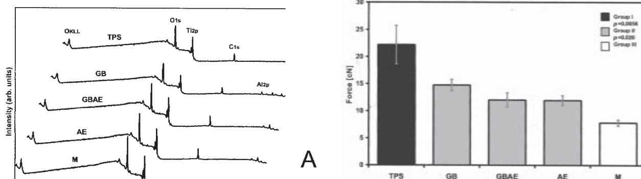
Figure 10 A. Low resolution X-ray photoelectron (XPS) spectroscopy of cpTi surfaces. Staggered depiction of the XPS binding energy profiles for cpTi surfaces. TPS: plasma-sprayed; GB: grit-blasted; GBAE: grit-blasted and dual acid-etched; AE: dual acid-etched; M: machined. Titanium oxide (Ti2p, Ti3p, OKLL, O1s), as well as residual carbon (C1s) are detected at all surfaces. At the GB surface, the additional presence of alumina (Al2p) is detected, which is due to residual Al_2O_3 particles from the grit blasting procedure.
